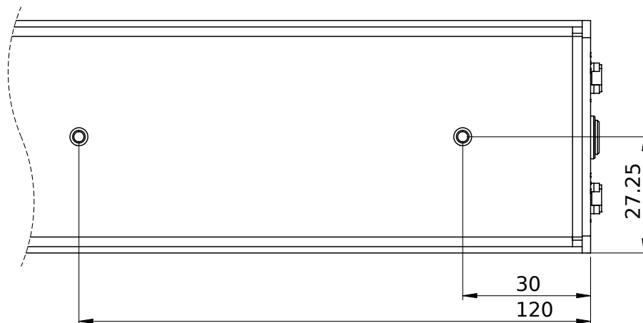
Figure 11: Mounting points for ACQ1002S (Stack) Case
