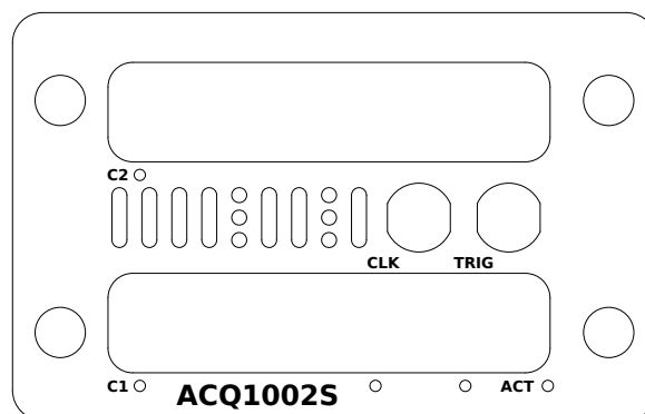
Figure 2: ACQ1002S Front Panel Stack
