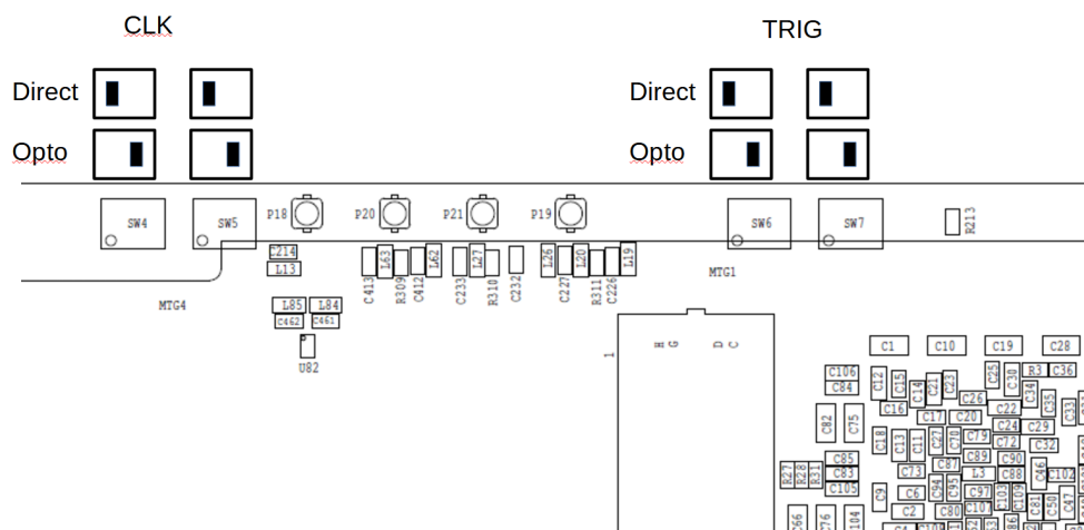
Figure 4: Opto-Coupler Switches
